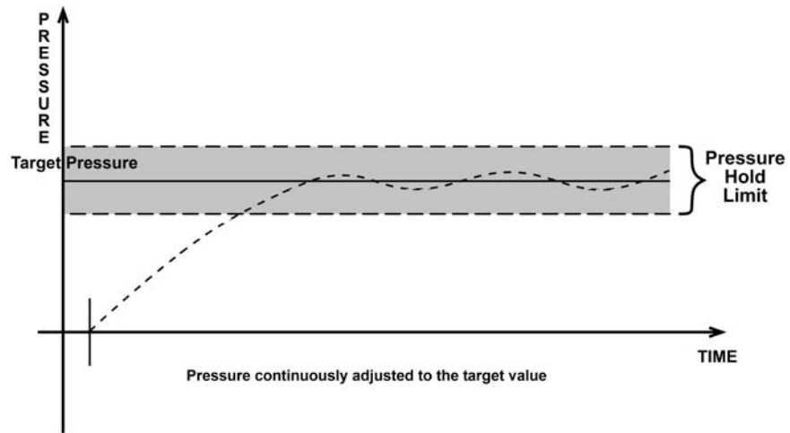
Figure 9. Dynamic Pressure Control Operation
