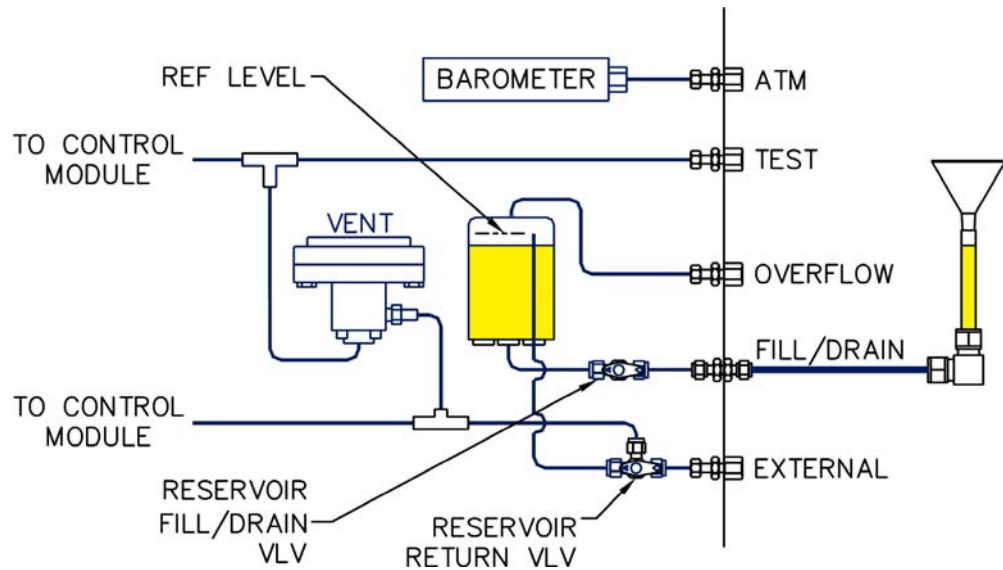
Figure 18. Internal Reservoir Schematic
