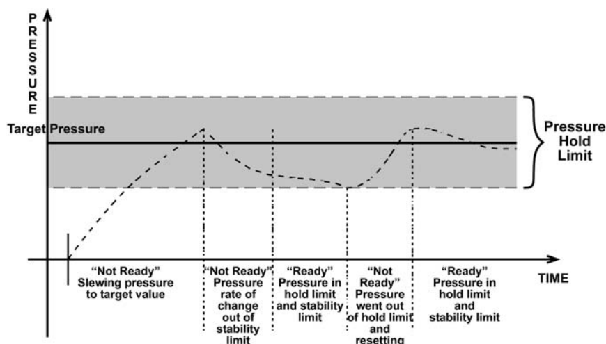
Figure 12. Ready/Not Ready in Static Control Mode
