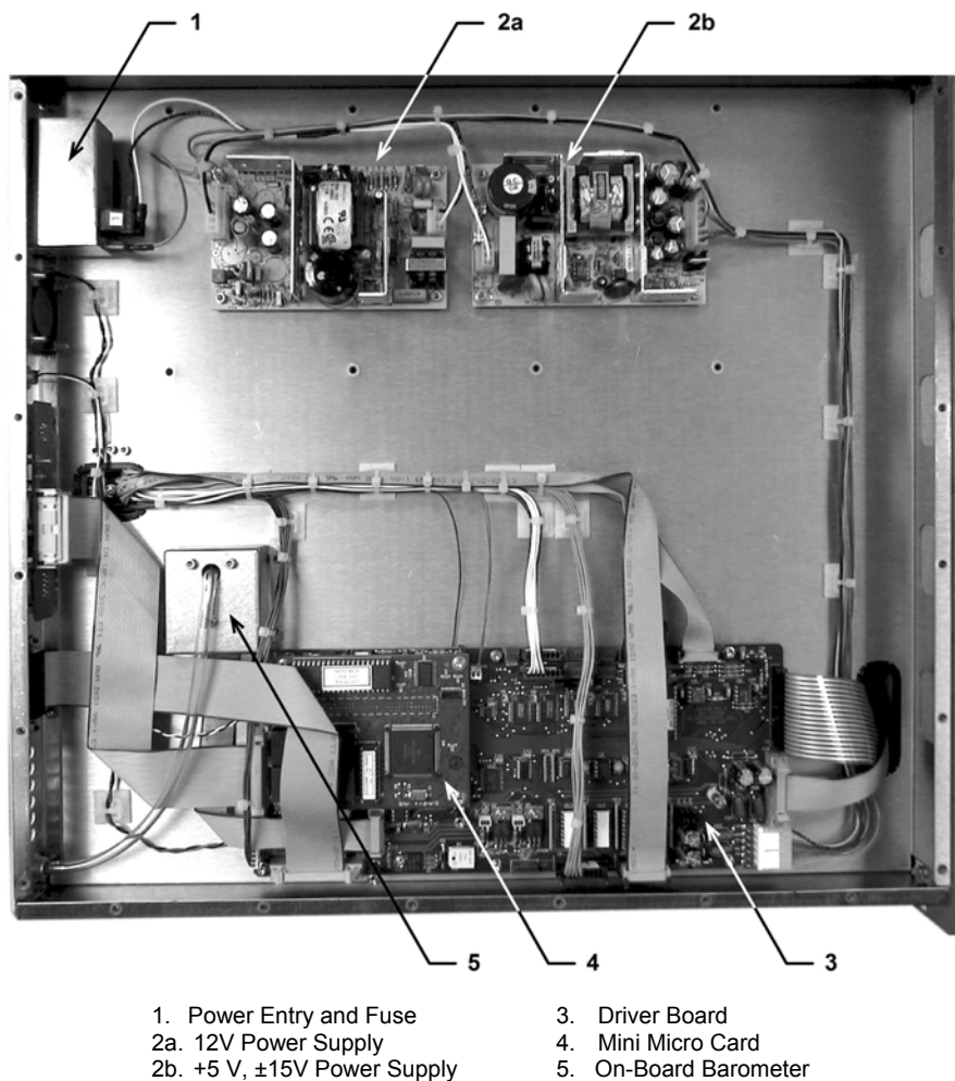
Figure 20. Electronic Module, Internal View
