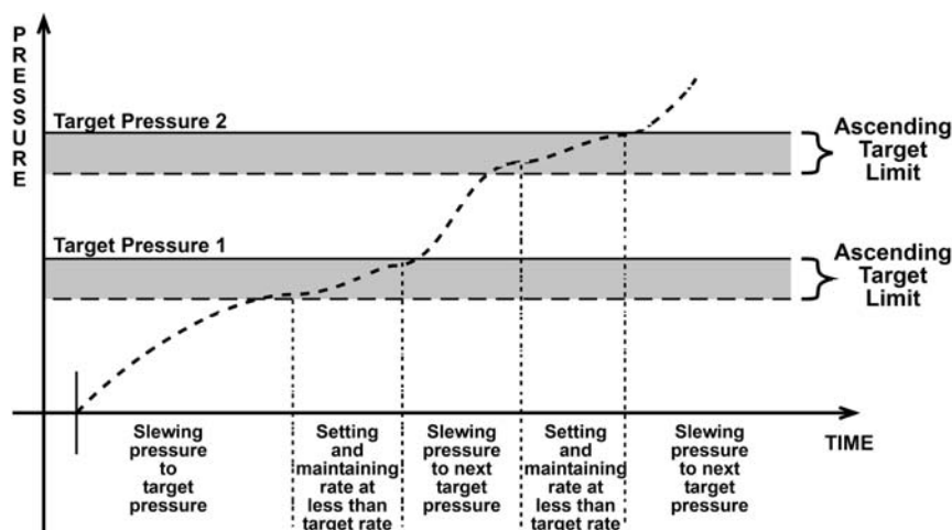
Figure 13. Monotonic Pressure Control Operation
