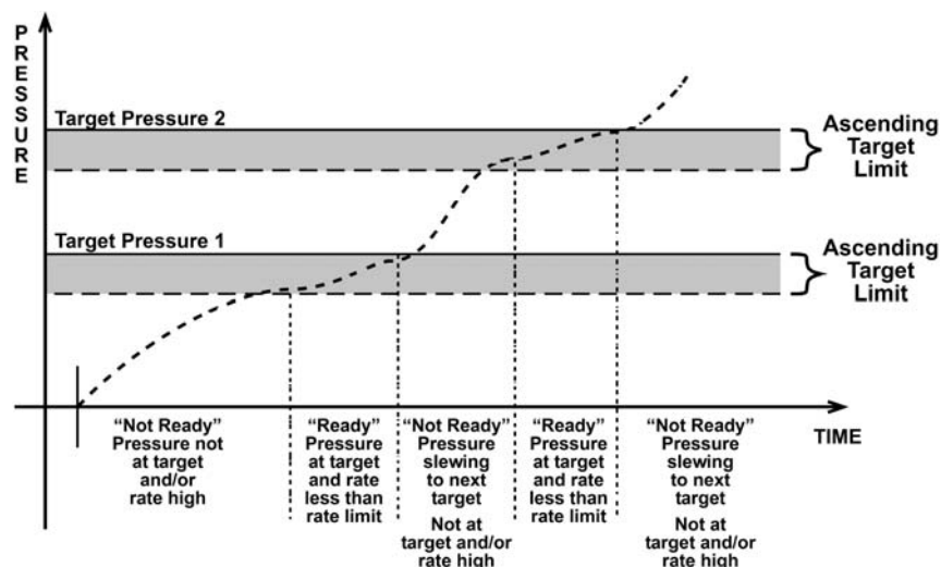
Figure 14. Ready/Not Ready in Monotonic Pressure Control Mode
