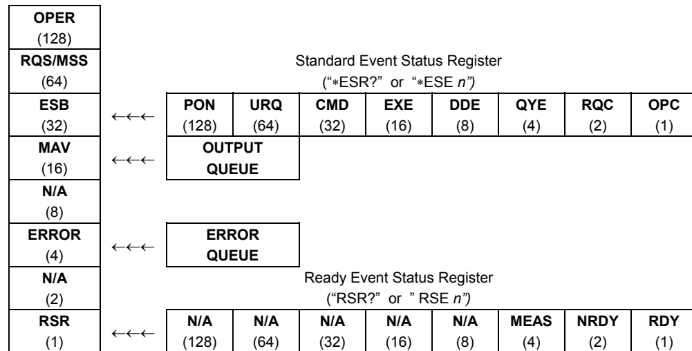
Figure 17. Status Register Schematic
