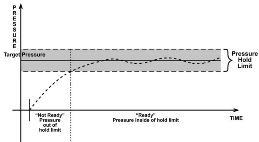
Figure 10. Ready/Not Ready in Dynamic Pressure Control Mode
