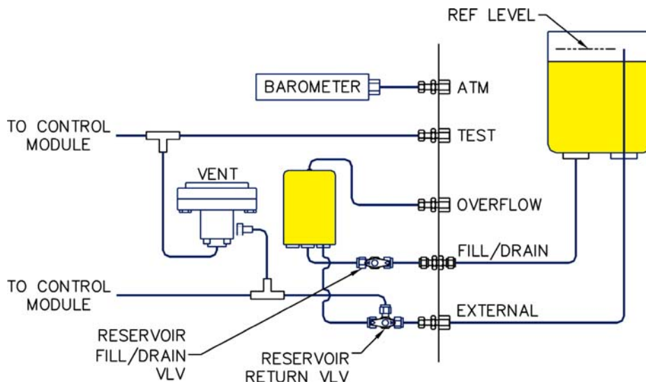
Figure 19. External Reservoir Schematic
