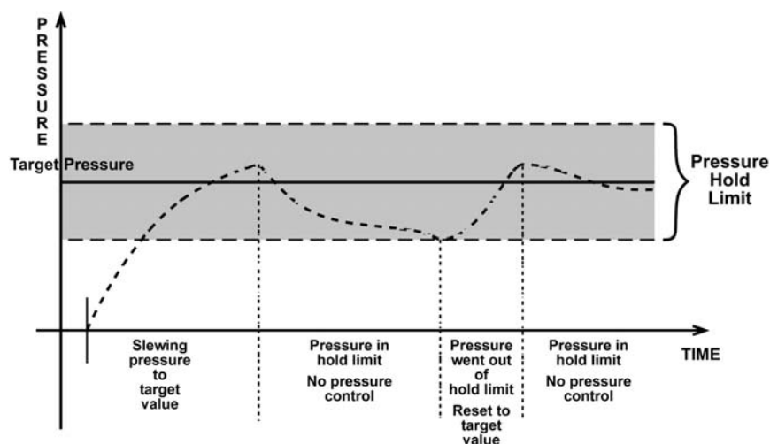
Figure 11. Static Pressure Control Operation
