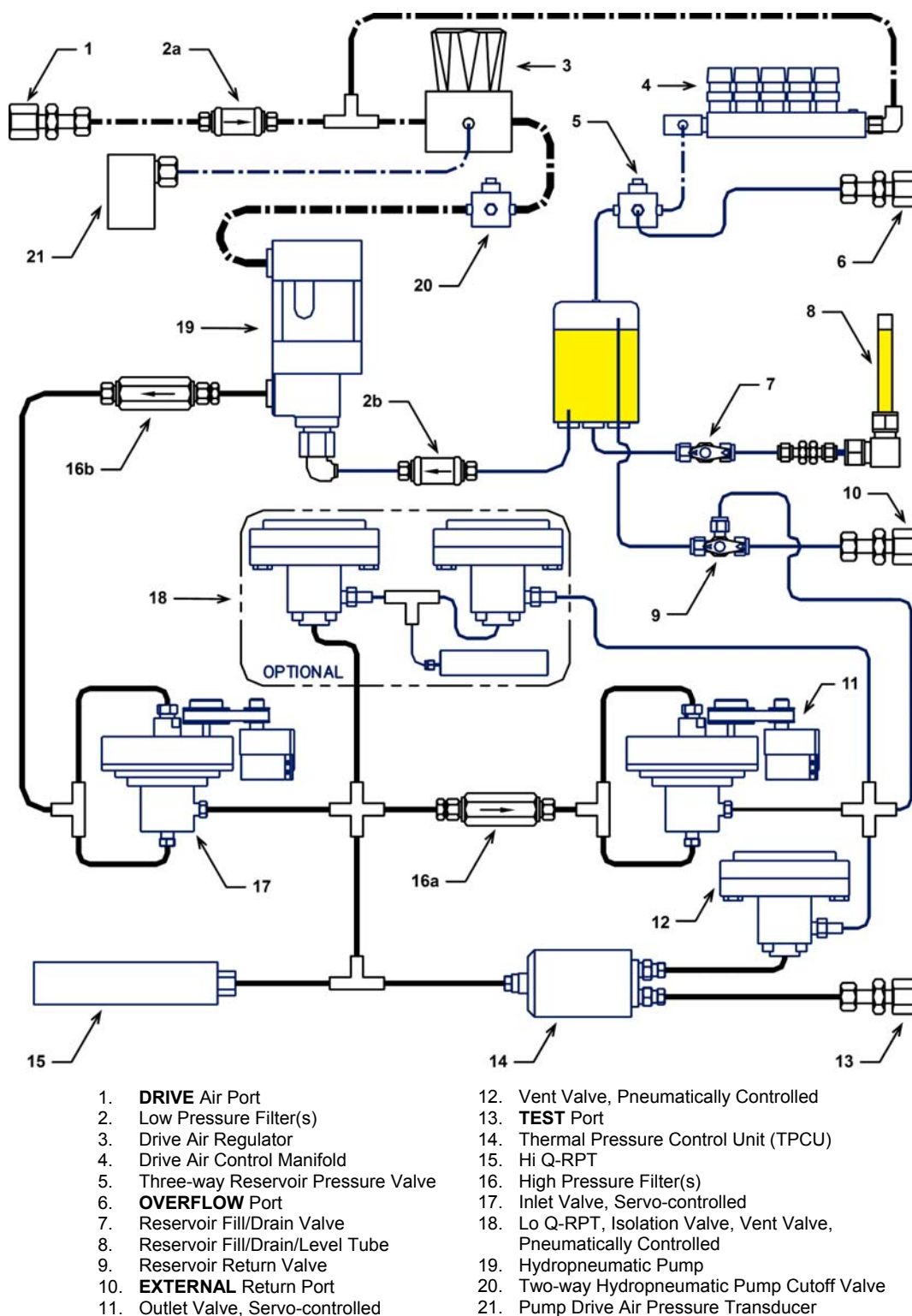
Figure 8. Pressure Control System Schematic
