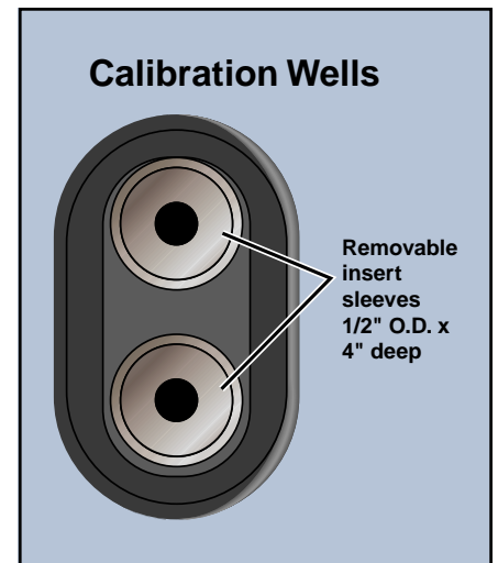
9102 block configuration. Instrument includes 1/4" and 3/16" inserts. Order additional sizes as needed.
