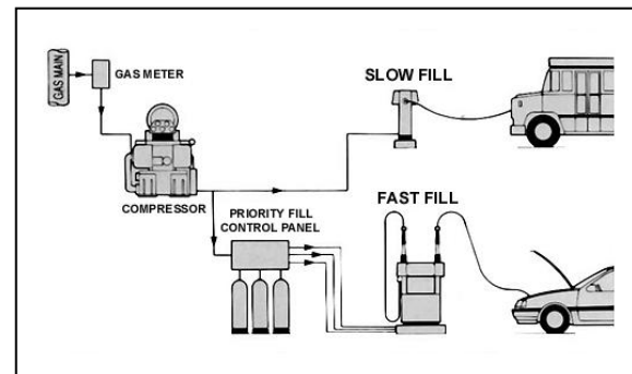
Typical CNG filling station layout
