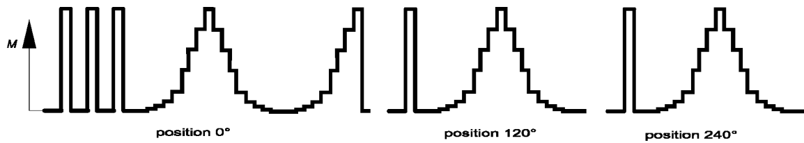
Fig. D.1: Example of preloadings and sequences for torque measuring devices with a minimum 8 steps and U < 0.1\%
