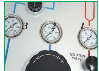
The MNR 90 precision volume adjuster allows very fine pressure control up to within 100 Pa
